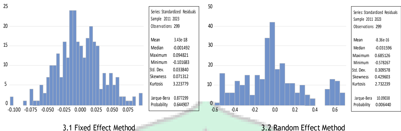
Figure 3. Histogram-normality Test
