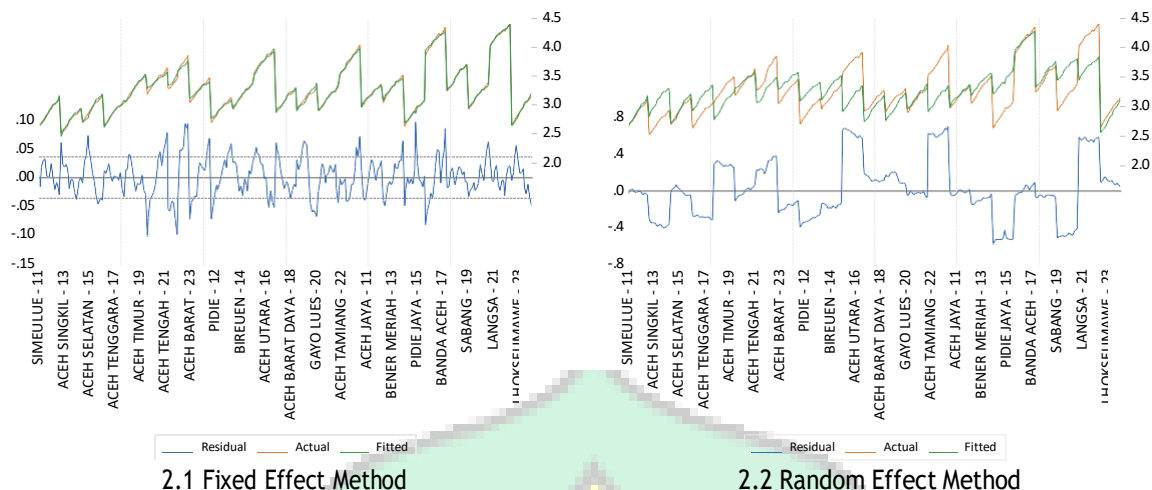
Figure 2. Residual Graph
