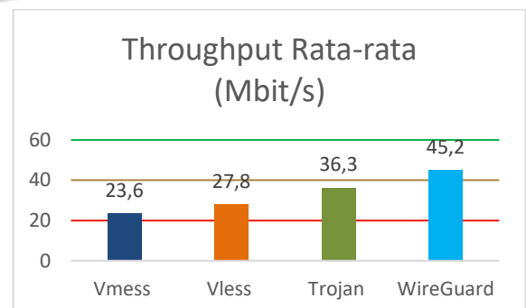
Gambar 5 Throughput Rata-rata
