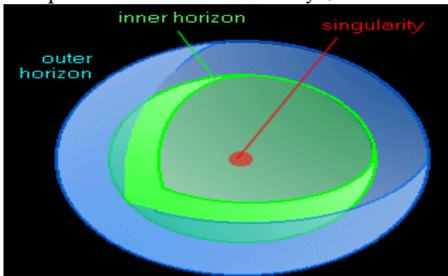
Gambar 3.2 Struktur Black-hole Reissner-Nordstrom. (Sumber: IN. Rumiuno)
