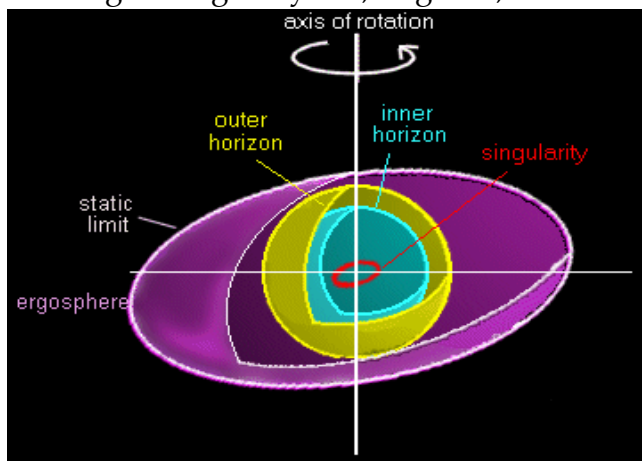
Gambar 3.3 Struktur Kerr Black-Hole
