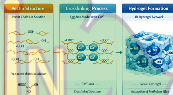
Gambar 4. Ilustrasi Adsorpsi
