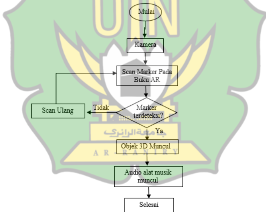
Gambar 2. Flowchart Media Edukasi
