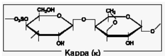
Figure 1:[ caragenan formula]
